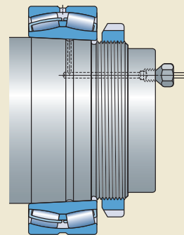
Dismounting a bearing from a tapered journal using the SKF oil injection method
