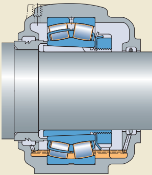
Spherical roller bearing application lubricated by an oil bath
