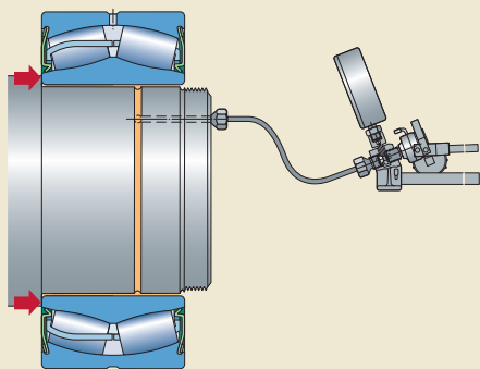
Dismounting a bearing from a cylindrical seating using the SKF oil injection method
